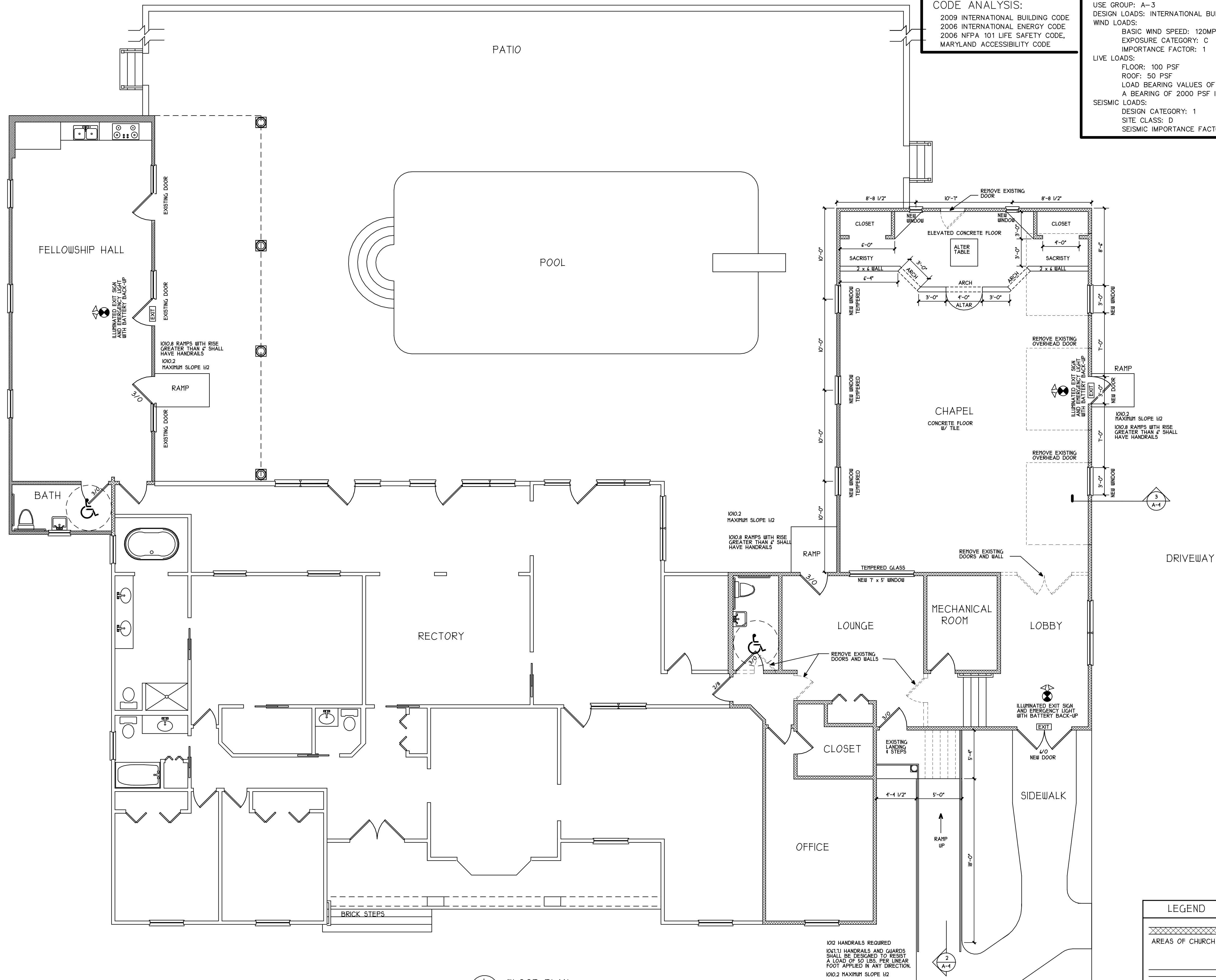
1 FLOOR PLAN A-3 3/16" = 1'
